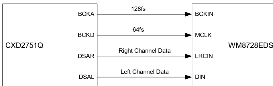
Figure 34 Biphas Mode Connection Diagram
