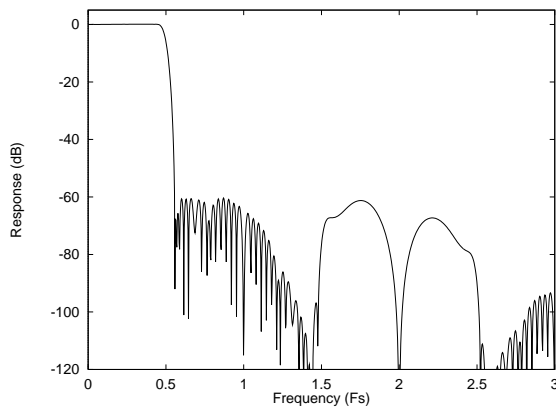
Figure 17 DAC Digital Filter Frequency Response -44.1, 48 and 96kHz
