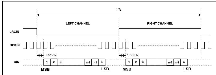
Figure 10 I 2 S Mode Timing Diagram
