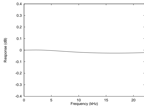
Figure 24 De-Emphasis Error (44.1kHz)
