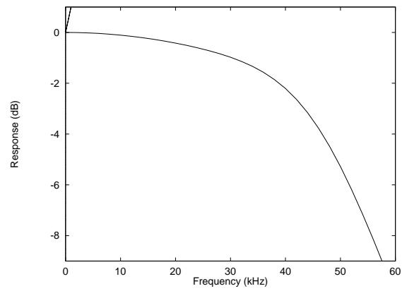
Figure 30 DSD frequency response - 4th order post filter
