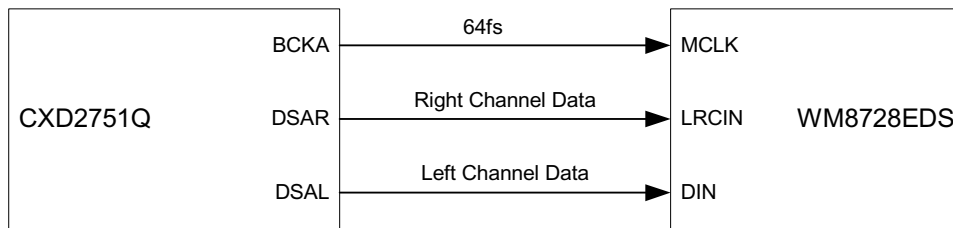
Figure 33 Monophase Mode Connection Diagram
