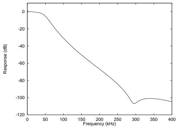
Figure 29 DSD frequency response - 4th order post filter
