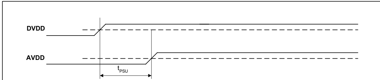
Figure 4 Power Supply Timing Requirements
