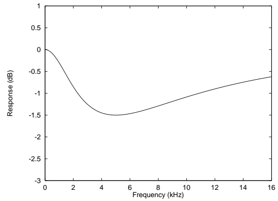
Figure 22 De-Emphasis Error (32kHz)
