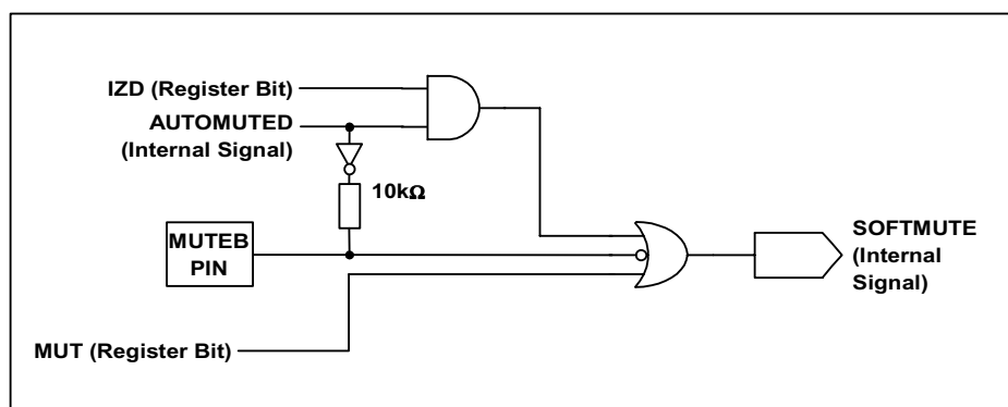
Figure 14 Selection Logic for MUTE Modes
