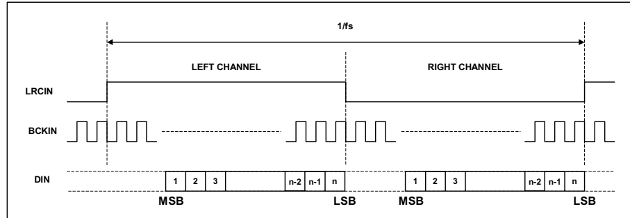
Figure 9 Right Justified Mode Timing Diagram
