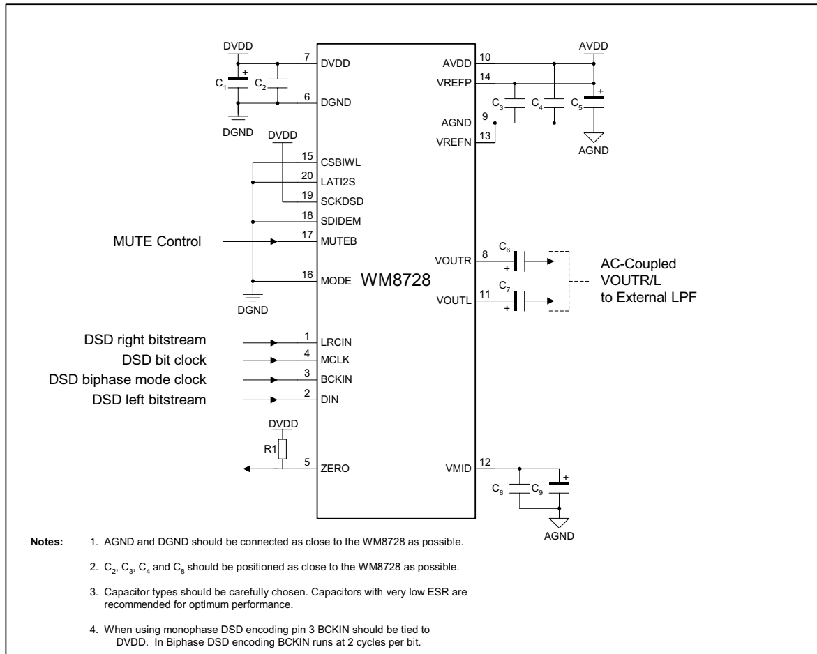
Figure 32 External Connections for DSD Applications
