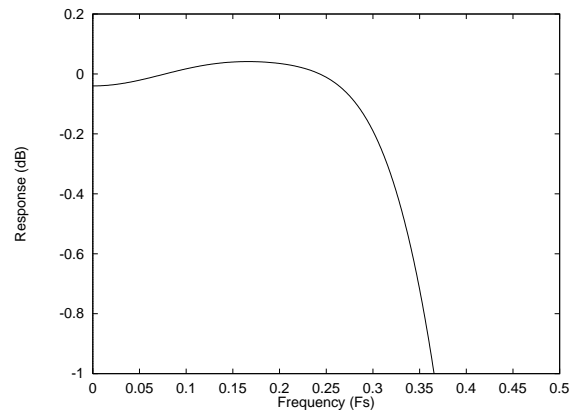
Figure 20 DAC Digital Filter Ripple -192kHz
