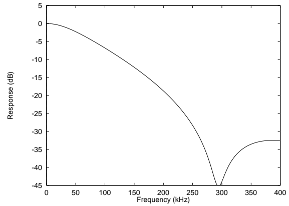
Figure 28 DSD Frequency Response - no post filter
