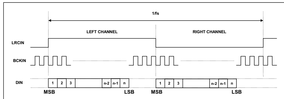
Figure 8 Left Justified Mode Timing Diagram
