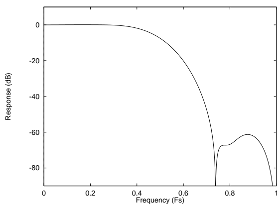
Figure 19 DAC Digital Filter Frequency Response -192kHz
