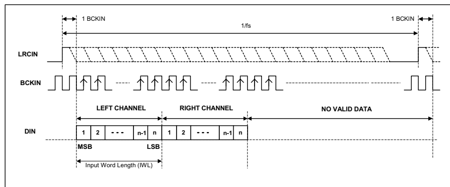
Figure 11 DSP Early Mode Timing Diagram
