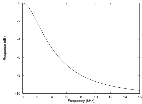
Figure 21 De-Emphasis Frequency Response (32kHz)
