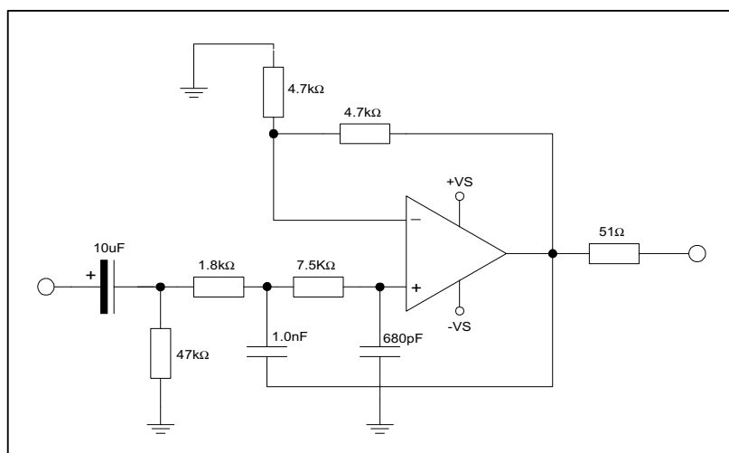
Figure 35 Recommended Low Pass Filter (Optional)
