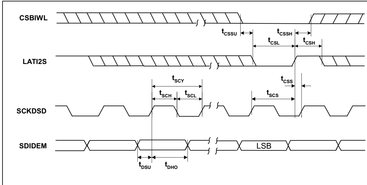
Figure 6 Program Register Input Timing - 3-Wire Serial Control Mode
