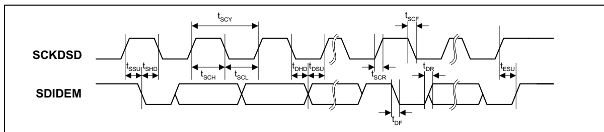
Figure 7 Program Register Input Timing - 2-Wire Serial Control Mode
