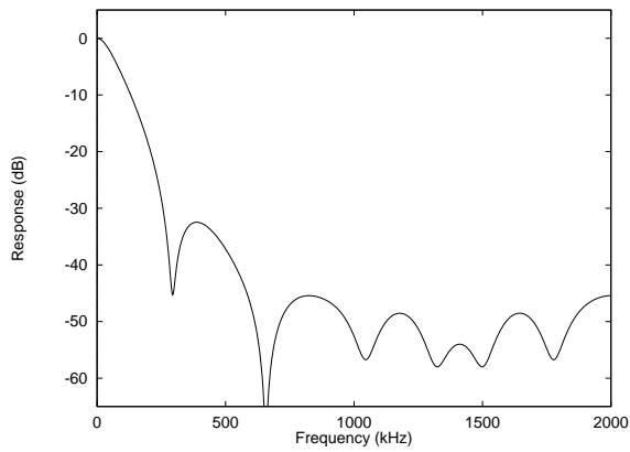
Figure 27 DSD Frequency Response - no post filter
