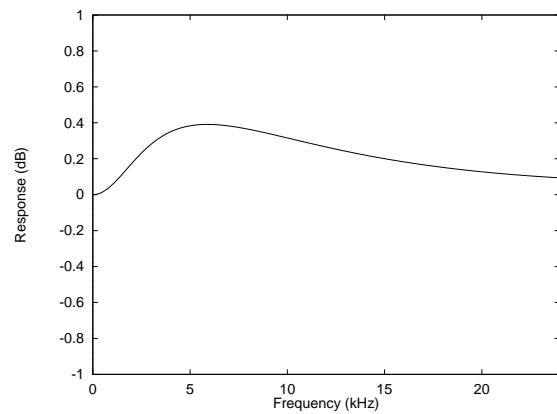
Figure 26 De-Emphasis Error (48kHz)
