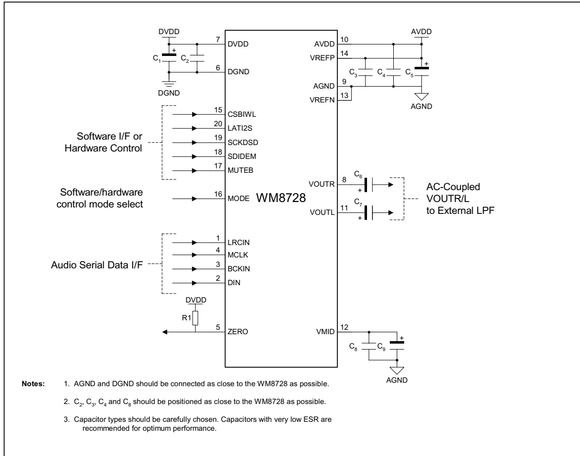
Figure 31 External Components Diagram
