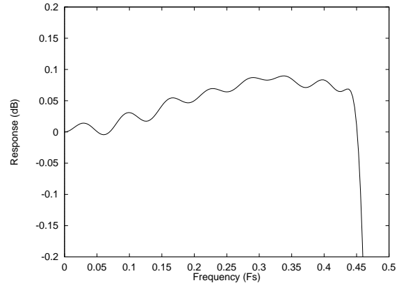
Figure 18 DAC Digital Filter Ripple -44.1, 48 and 96kHz
