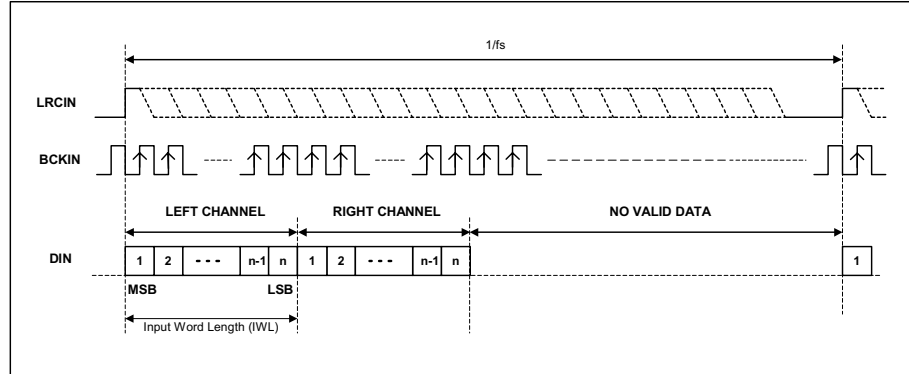
Figure 12 DSP Late Mode Timing Diagram
