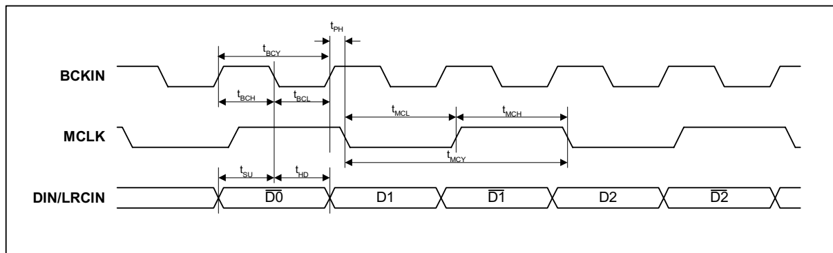
Figure 5 Biphas DSD Timing Requirements
