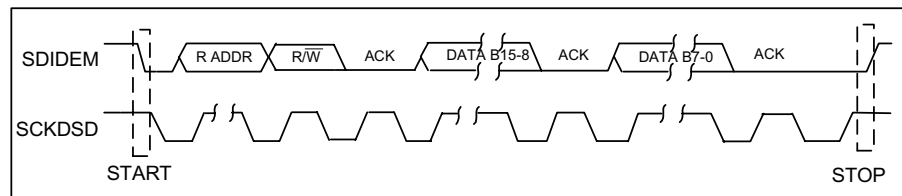
Figure 16 2-Wire Serial Interface
